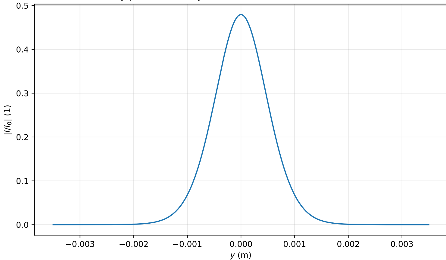
Intensity profile I(x = 0, y, z = 3.025)/I_0 , P_{in}=0.4P_{cr} , artificial time
